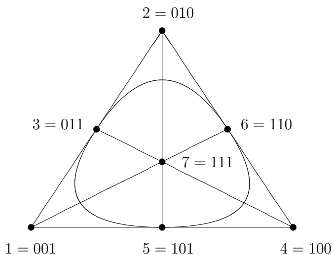
FIGURE 2. The projective space \text{PG}(2, 2) .
